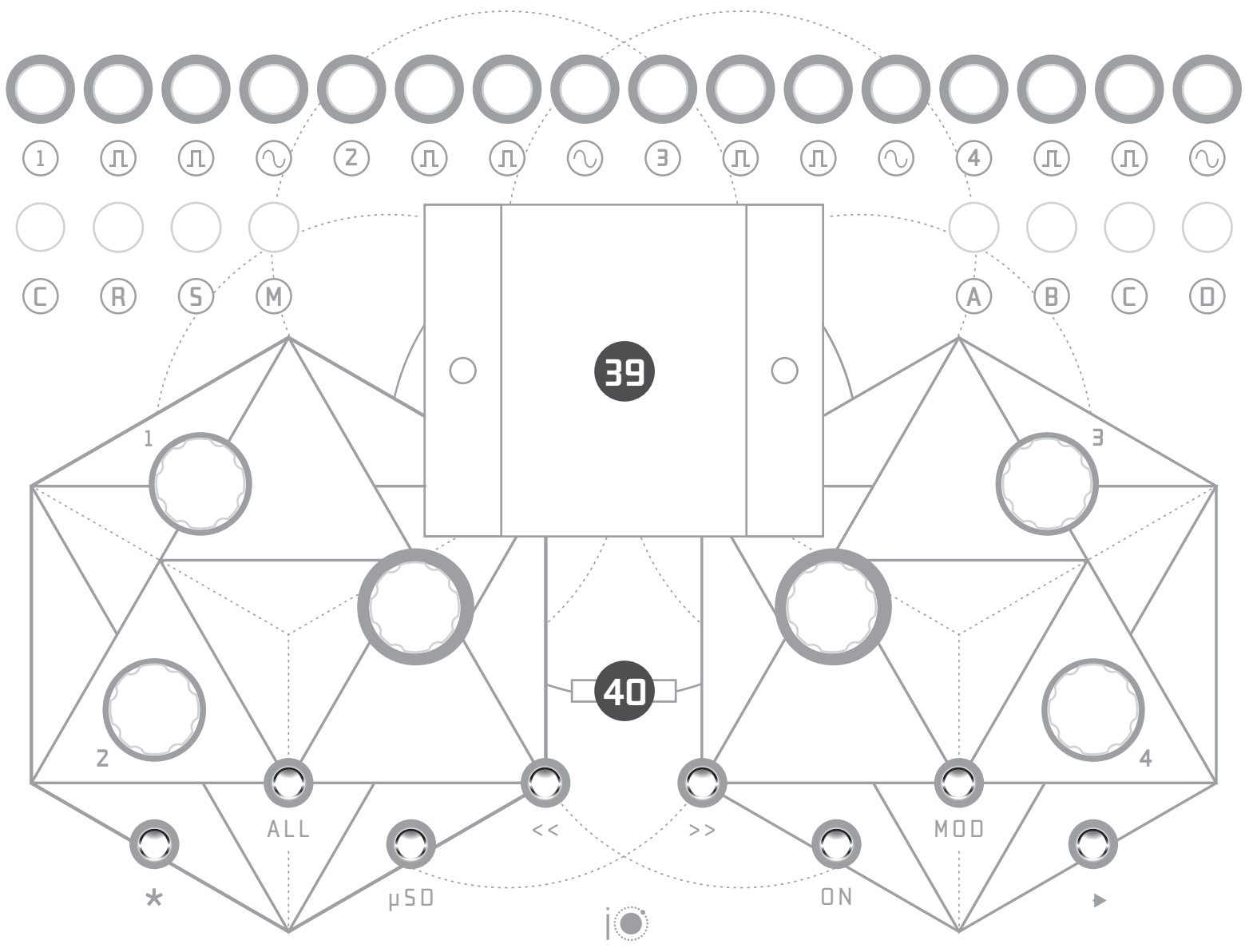
39: UI Display 40: Micro SD Card Slot
